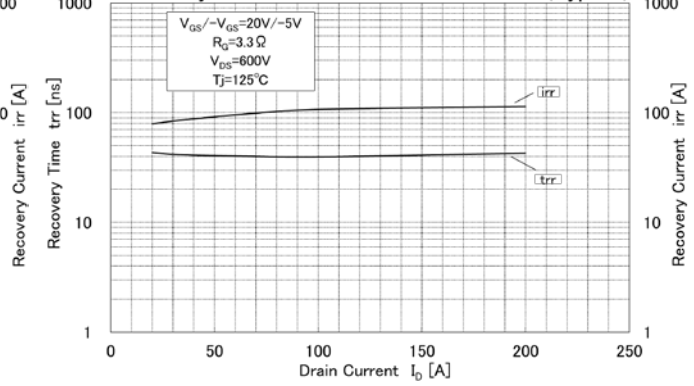
Recovery Characteristics vs. Drain Current (Typical)
